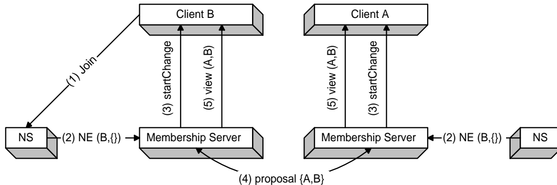
Figure 2: The membership service typical message flow.
