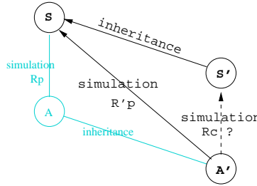
Fig. 5. Intermediate step: Reusing R'_p for building R_c .
