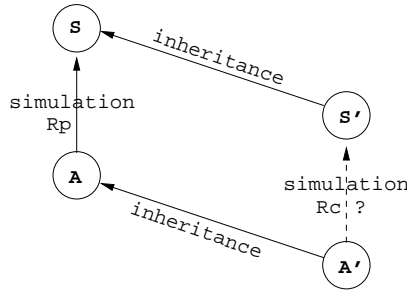
Fig. 1. Algorithm A simulates specification S with R_p . Can R_p be reused for building a simulation R_c from a child A' of A to a child S' of S ?
