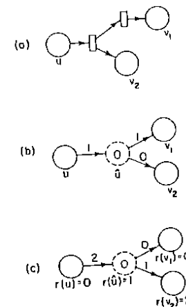
Fig. 5. Modeling two-way fanout with an extra vertex having delay zero.
