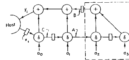
Fig. 2. Correlator 2: a retimed circuit functionally equivalent to, but more efficient than, Correlator 1. The longest path of combinational rippling begins at the register on connection C , and the clock period of this circuit is 17 esec.
