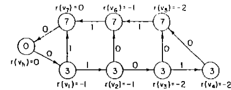
Fig. 4. The graph model of an optimal correlator with clock period 13. The circuit is obtained from the graph of Correlator 1 in Figure 3 by applying the optimal retiming, determined by Algorithm OPT1. For each vertex v , the value r(v) is the lag of v with respect to the corresponding vertex in Correlator 1. The retimed weight of an edge u \xrightarrow{e} v is given by w_r(e) = w(e) + r(v) - r(u) .
