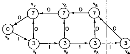
Fig. 3. The graph model of Correlator 1 from Figure 1.
