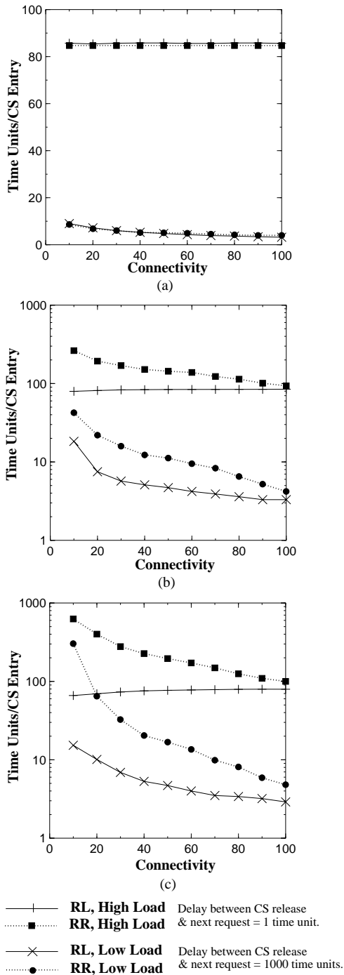
Figure 10. Connectivity vs. time per CS entry for (a) zero, (b) low ( \lambda_{mob} = 5 \times 10^{-2} ), and (c) high ( \lambda_{mob} = 5 \times 10^{-1} ) mobility in RL vs. RR simulations.
