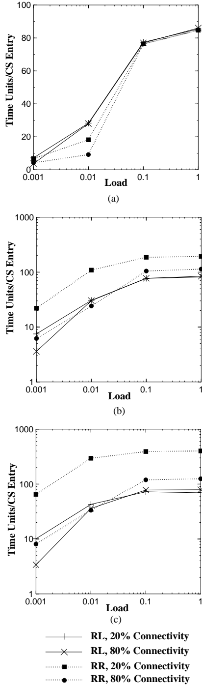
Figure 9. Load vs. time per CS entry for (a) zero, (b) low ( \lambda_{mob} = 5 \times 10^{-2} ), and (c) high ( \lambda_{mob} = 5 \times 10^{-1} ) mobility in RL vs. RR simulations.
