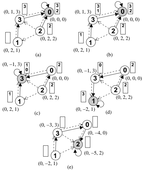
Figure 7. Operation of reverse link mutual exclusion algorithm on static network.
