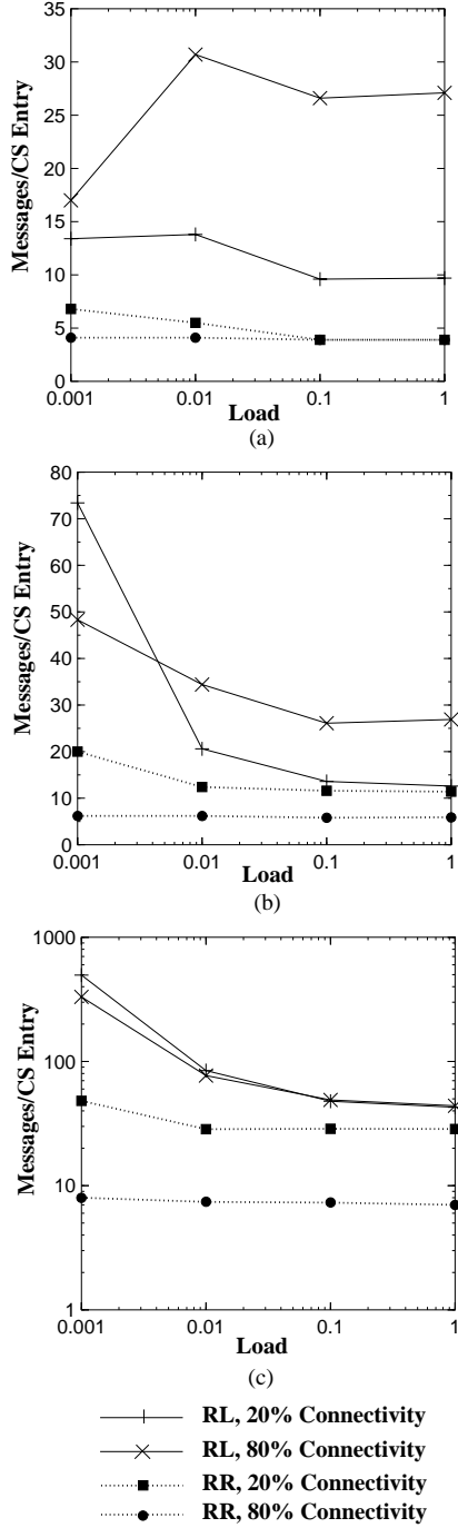
Figure 11. Load vs. messages per CS entry for (a) zero, (b) low ( \lambda_{mob} = 5 \times 10^{-2} ), and (c) high ( \lambda_{mob} = 5 \times 10^{-1} ) mobility in RL vs. RR simulations.
