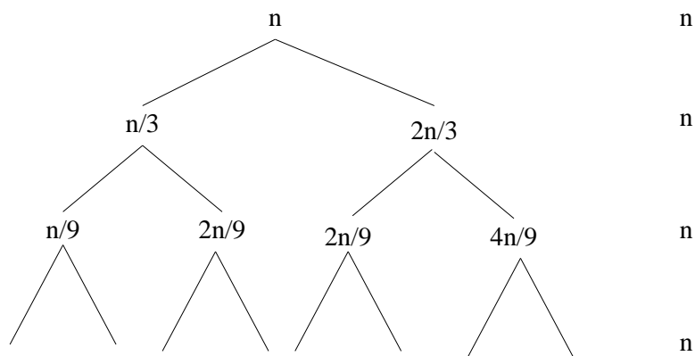
Figure 1: Recursion tree
