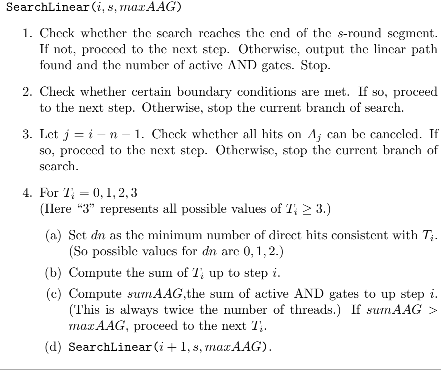
Figure 6.9: Algorithmic procedure to search for valid linear paths.
