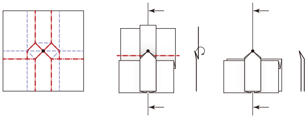
Fig. 8 The thorn gadget folds an infinite sheet of paper (left) into a plane with a small triangular tab (middle). The gadget is composed of 27 creases and 19 faces, so it is an all-layers flat folding step of complexity 18.
