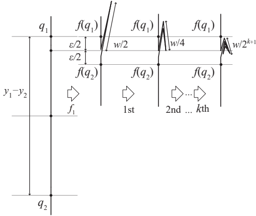
Fig. 12 Parallel shrink folding: reducing a horizontal strip down to small height.
