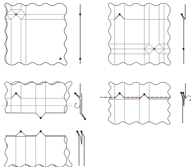
Fig. 9 The folding sequence for infinite paper, crease passing case. Each flat folding step has complexity O(1) . The final folding step is a simple fold/unfold as drawn, but by shifting the fold line up slightly, it is a simple fold.
