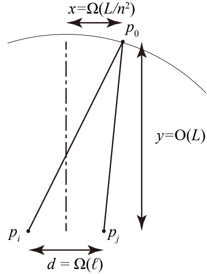
Fig. 5 Analyzing the radial feature ratio in Lemma 3.8.
