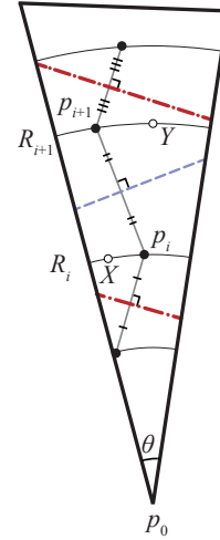
Fig. 11 Each bisector lies between adjacent arcs.
