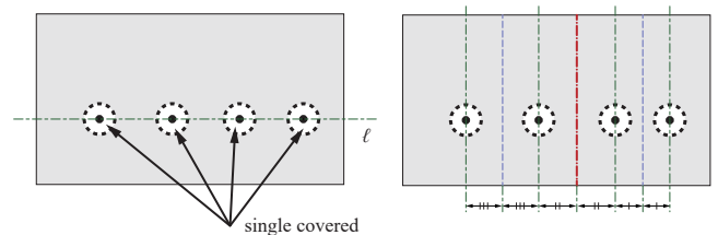
Fig. 4 Bisection folding to align collinear points.
