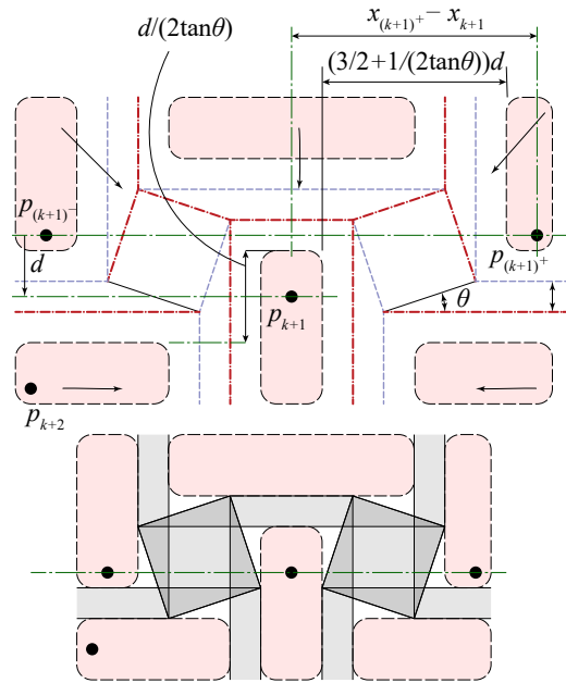
Fig. 13 Downshifting gadget can be inserted if conditions (i)–(ii) are satisfied.
