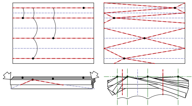
Fig. 6 If we fold the paper by mountain creases y = y_i ( 1 \leq i \leq n ) and valley creases y = (y_i + y_{i+1})/2 ( 1 \leq i \leq n - 1 ), we get the product on the left side. If we reverse-fold each mountain by a sufficiently small angle at p_i , we get the product on the right side. In either case, the p_i 's are all on a horizontal line, and in the latter case, no other points cover these points.
