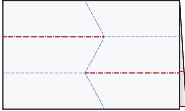
Fig. 3 An example of an all-layers flat folding step of complexity 5.
