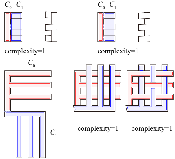
Fig. 2 Weaving with folding steps of complexity 1.
