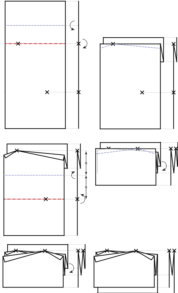
Fig. 7 How to fold Fig. 6 only by some-layers simple folds.
