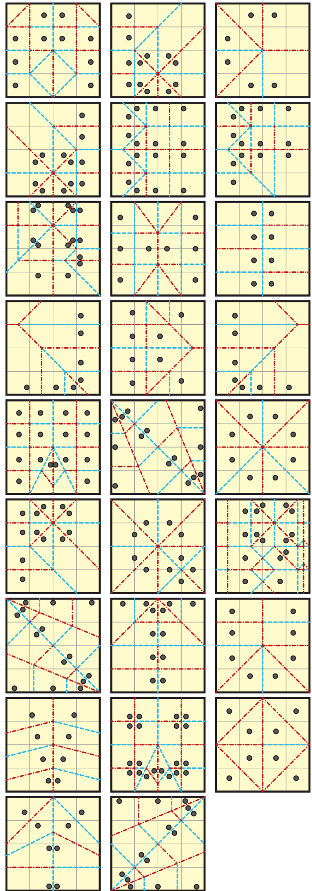
Fig. 1 Creating every letter of the alphabet by folding (along the specified crease pattern) and one punch, resulting in the circular holes. These foldings were designed by hand to be as simple as possible, using the ORIPA software. Amusingly, M and W use the same crease pattern, without rotation or reflection.
