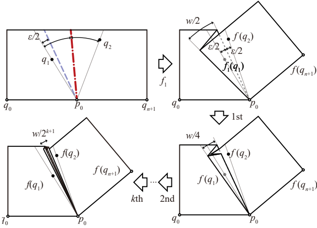
Fig. 10 Radial shrink folding: reducing a wedge down to a thin fan.
